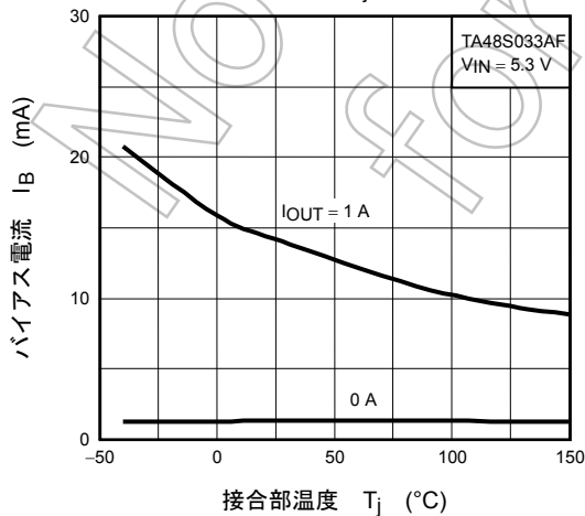
I_B - T_j
