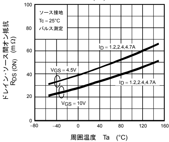
R_{DS(ON)} - T_a
