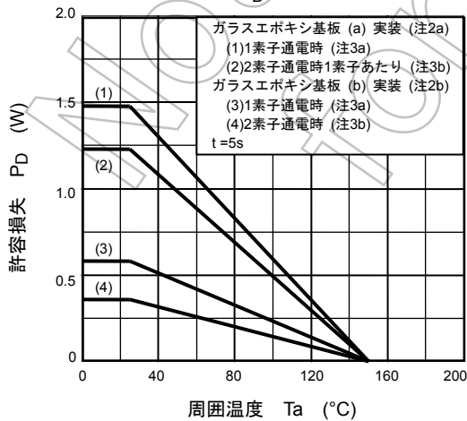
P_D - T_a
