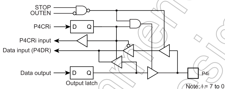
Figure 7-6 Port P4
