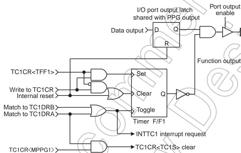
Figure 8-7 \overline{\text{PPG}} Output
