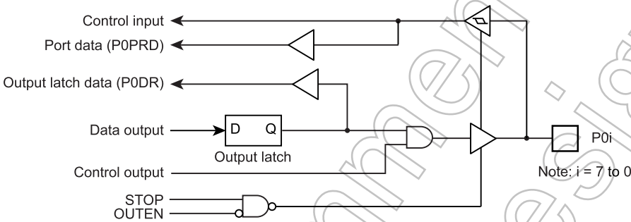
Figure 7-2 Port P0
