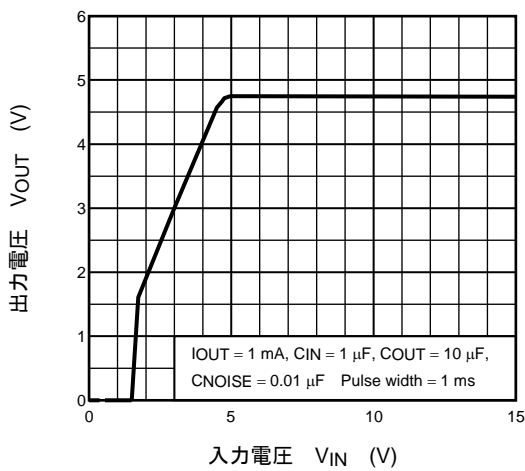
(TAR5SB48) V_{OUT} - V_{IN}
