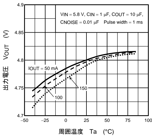
(TAR5SB48) V_{OUT} - T_a
