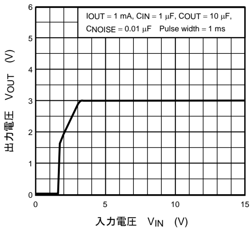
(TAR5SB30) V_{OUT} - V_{IN}
