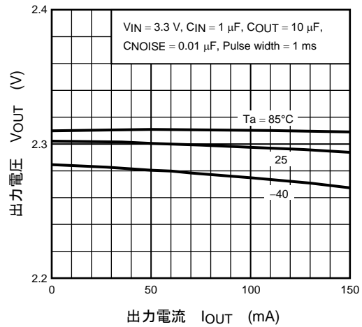
(TAR5SB23) I OUT - V OUT
