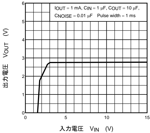
(TAR5SB28) V_{OUT} - V_{IN}
