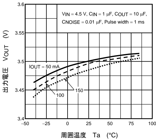
(TAR5SB35) V_{OUT} - T_a
