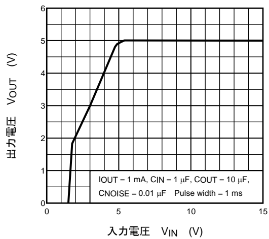
(TAR5SB50) V_{OUT} - V_{IN}
