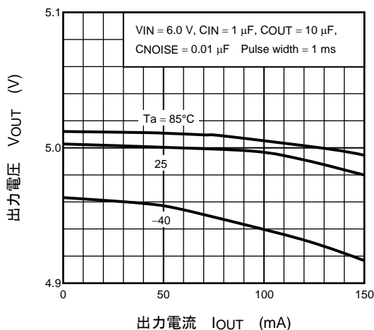
(TAR5SB50) I OUT - V OUT
