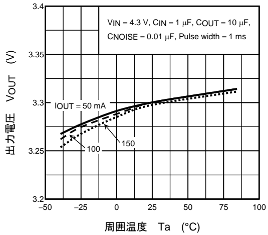
(TAR5SB33) V_{OUT} - T_a
