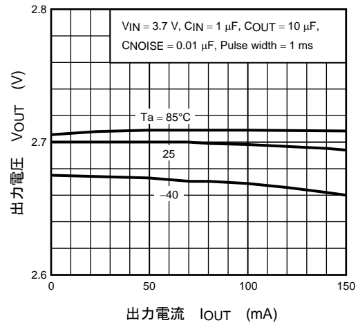
(TAR5SB27) I OUT - V OUT
