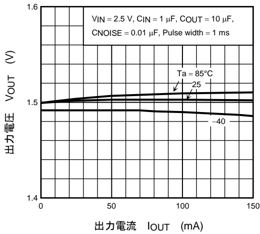
(TAR5SB15) I OUT - V OUT
