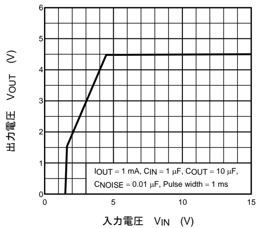
(TAR5SB45) V_{OUT} - V_{IN}
