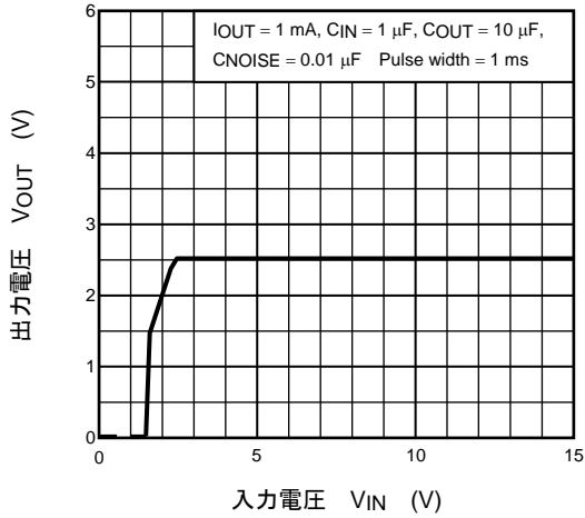
(TAR5SB25) V_{OUT} - V_{IN}
