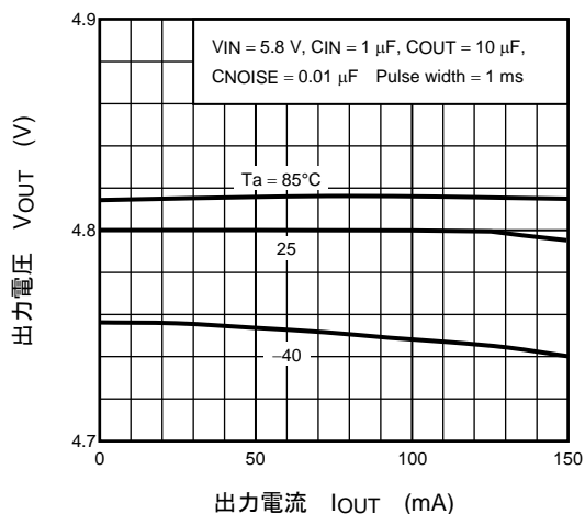
(TAR5SB48) I OUT - V OUT
