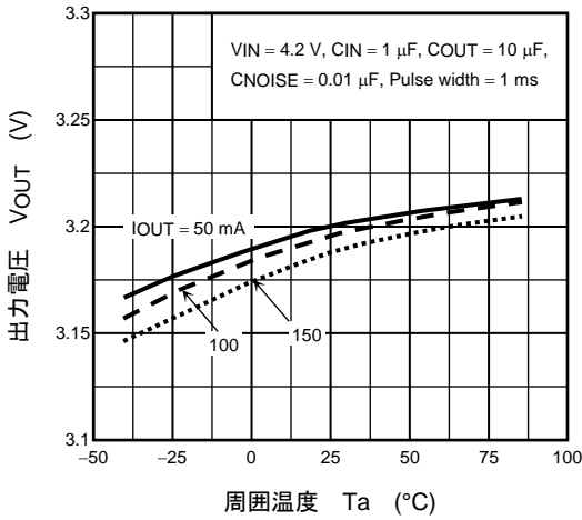
(TAR5SB32) V_{OUT} - T_a
