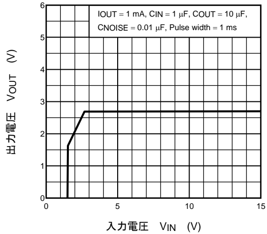
(TAR5SB27) V_{OUT} - V_{IN}
