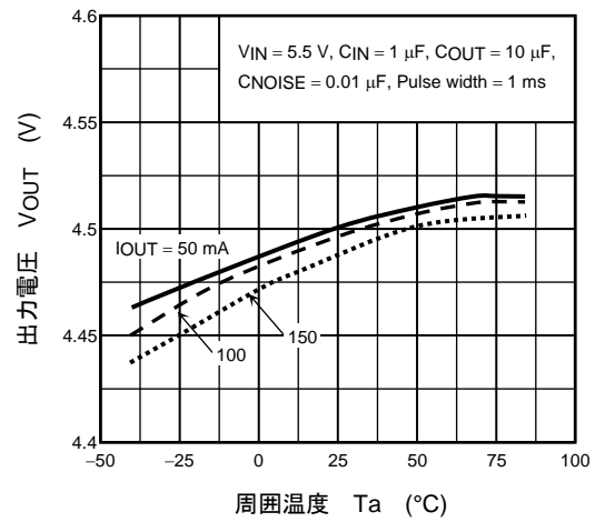
(TAR5SB45) V_{OUT} - T_a
