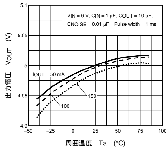
(TAR5SB50) V_{OUT} - T_a
