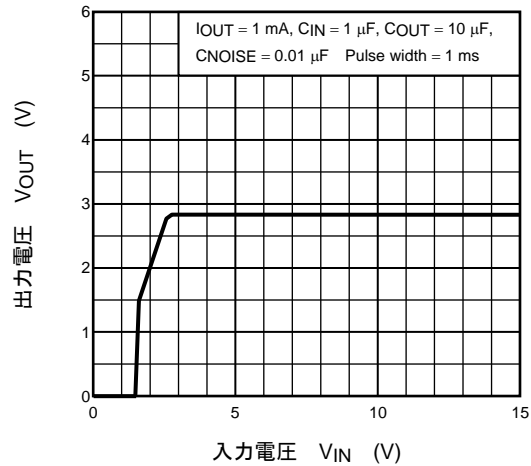
(TAR5SB29) V_{OUT} - V_{IN}
