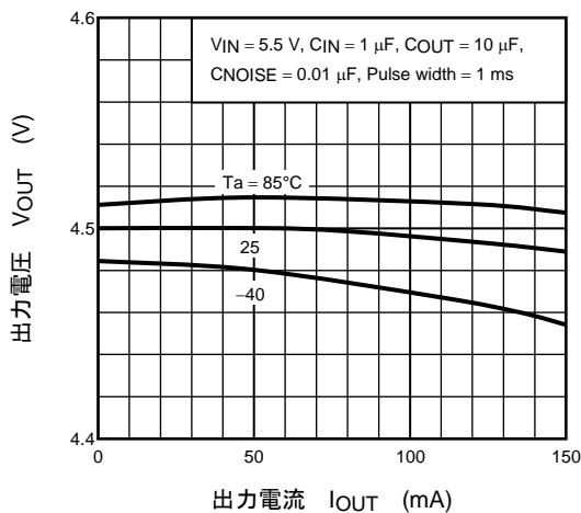
(TAR5SB45) I OUT - V OUT
