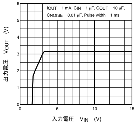
(TAR5SB31) V_{OUT} - V_{IN}
