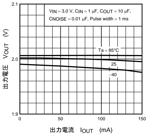
(TAR5SB20) I OUT - V OUT
