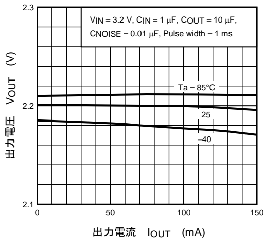
(TAR5SB22) I OUT - V OUT
