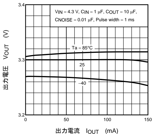
(TAR5SB33) I OUT - V OUT
