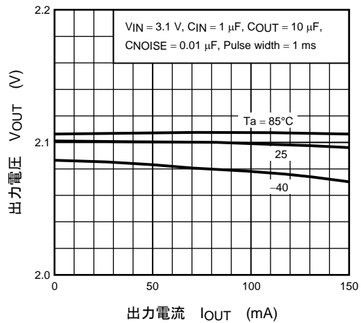
(TAR5SB21) I OUT - V OUT
