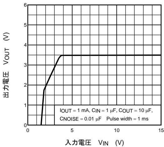
(TAR5SB35) V_{OUT} - V_{IN}
