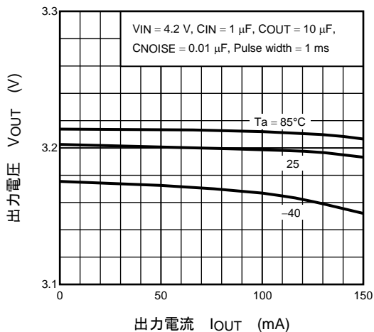
(TAR5SB32) I OUT - V OUT
