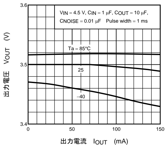
(TAR5SB35) I OUT - V OUT
