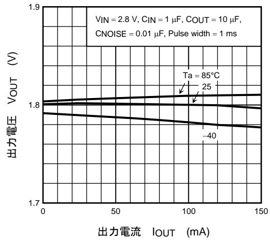
(TAR5SB18) I OUT - V OUT
