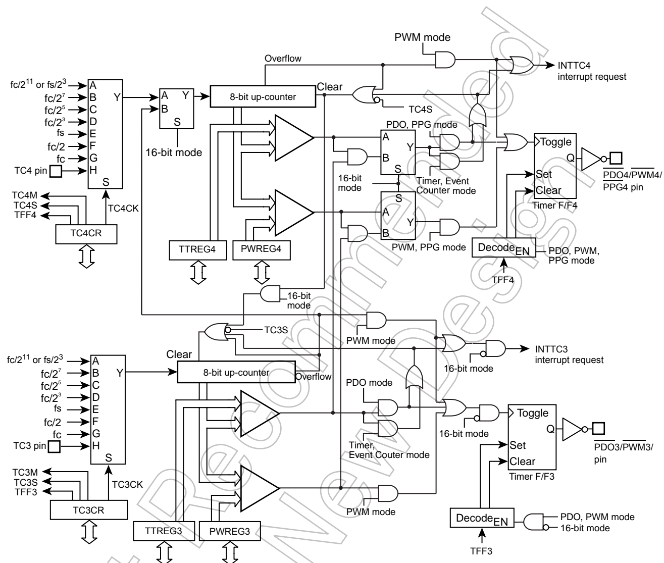
Figure 9-1 8-Bit TimerCounter 3, 4
