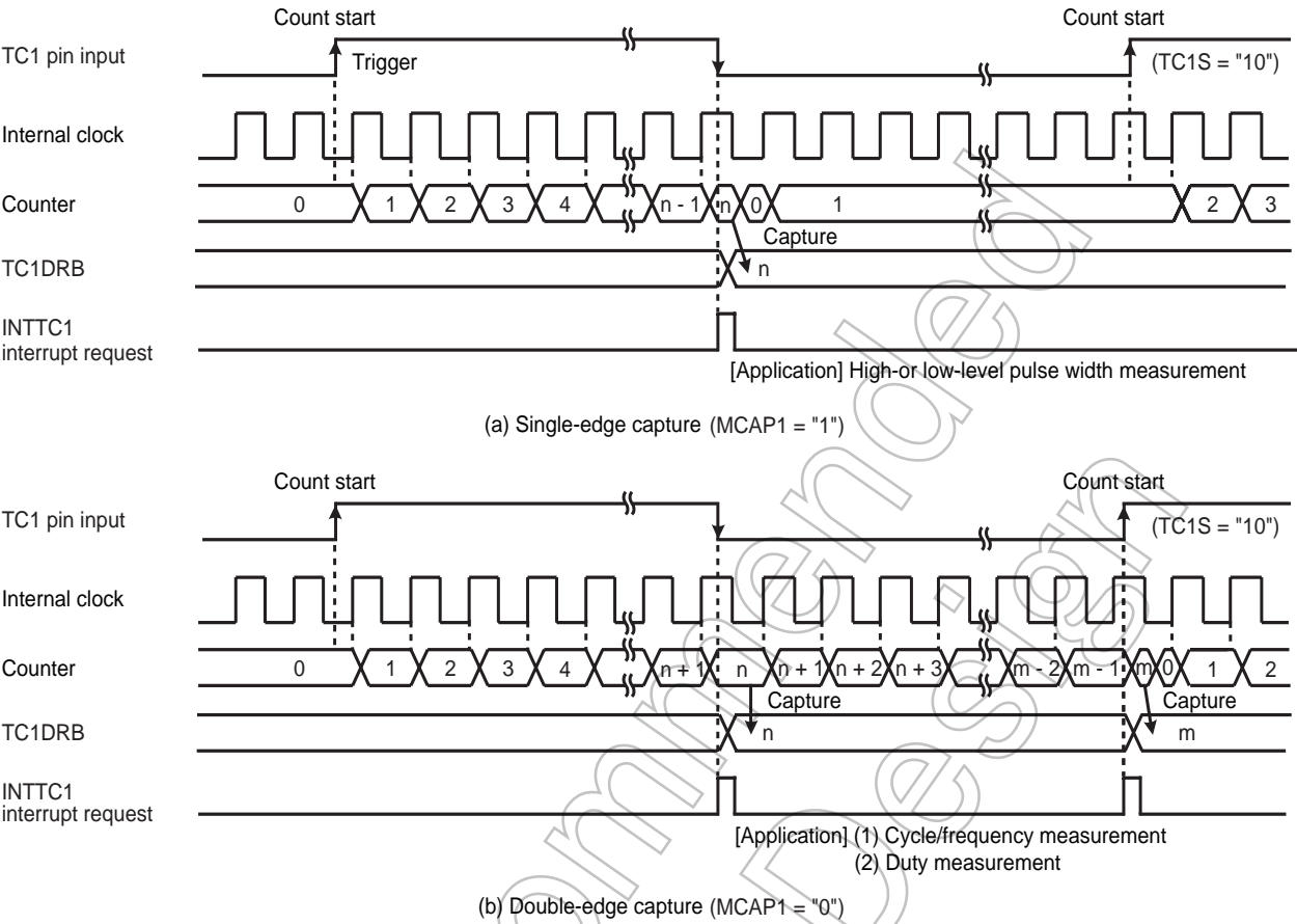
Figure 8-6 Pulse Width Measurement Mode
