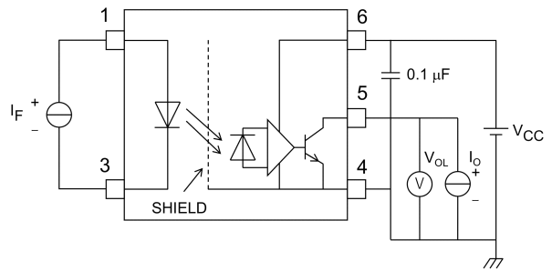
Fig. 12.1.2 V_{OL} Test Circuit
