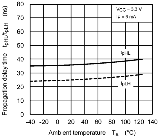
Fig. 12.2.9 t_{pHL}/t_{pLH} - T_a
