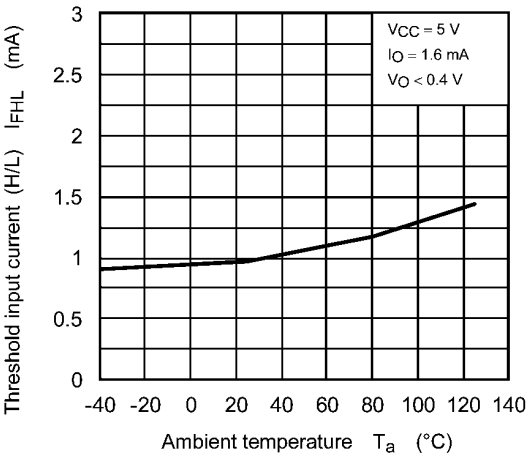
Fig. 12.2.8 I_{FHL} - T_a
