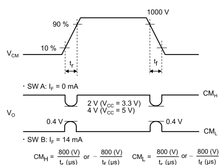
Fig. 12.1.6 Common-Mode Transient Immunity Test Circuit and Waveform
