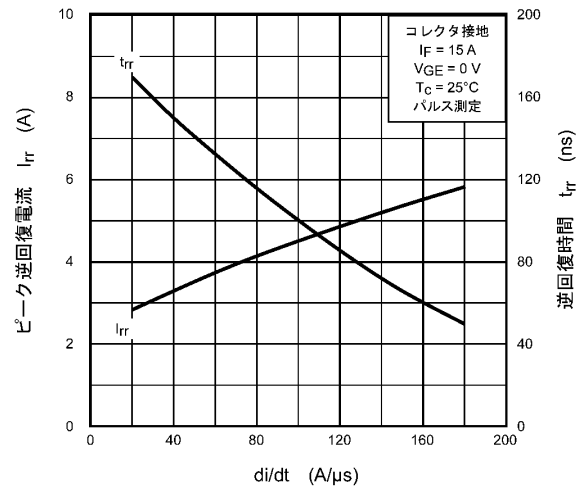
図 8.16 I rr , t rr - di/dt
