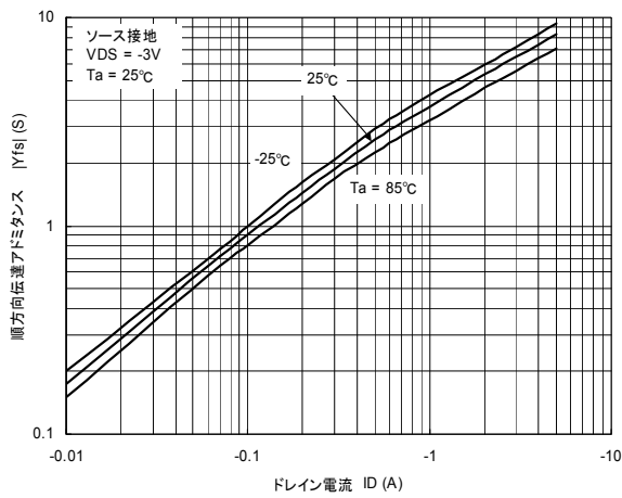
|Yfs| - ID
