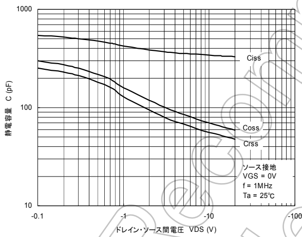
C - VDS
