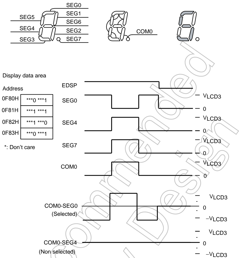
Figure 15-11 Static Drive
